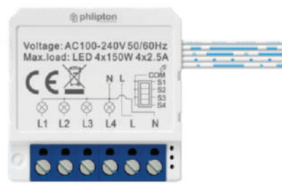
4 Gang ZigBee
